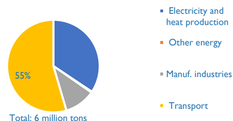
2020 Fuel Combustion CO 2 : % By Sector
