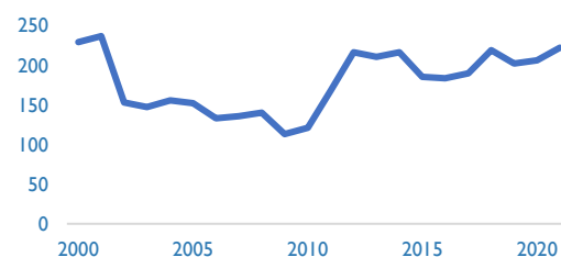
Armenia Historical Grid kgCO 2 /MWh
